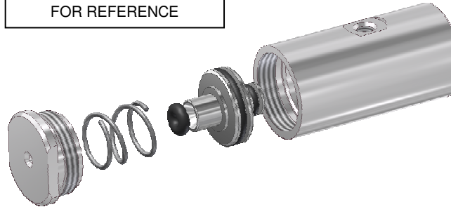
"ME001" EXPLODED VIEW FOR REFERENCE
